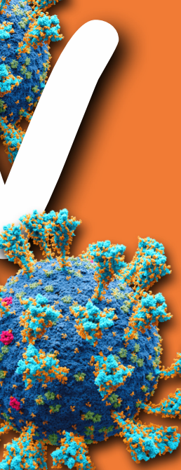
Virus
